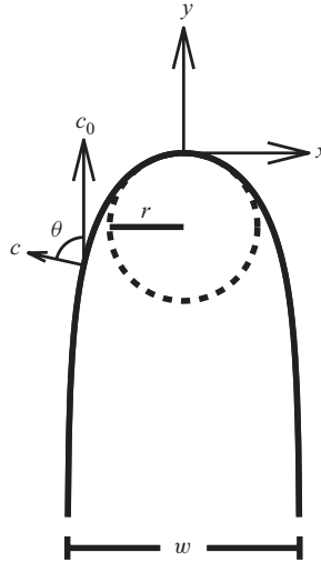
FIGURE 3. A balance between curvature-driven growth and translational growth sets the shape (5.2) of an amphitheatre-shaped valley head (solid black curve). When a curve evolves due to curvature-driven growth, the normal velocity c is inversely proportional to the radius of the best-fitting circle at that point. When a curve translates forward, there is a geometric relationship between the speed at which a point translates c_0 and the speed at which it grows in the normal direction c . This balance produces channels with a well-defined width w and an aspect ratio of w/r = \pi .
