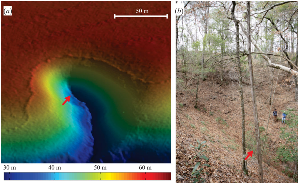
FIGURE 1. Examples of seepage valleys from the Florida network. (a) Topography obtained from a high-resolution map (Abrams et al. 2009) showing the rounded ‘amphitheatre-shaped’ valley head surrounding a spring (red arrow). Colours represent elevation above sea level. (b) A seepage valley head as viewed from the sidewall. The red arrow shows the approximate position of the spring. Note people for scale.
