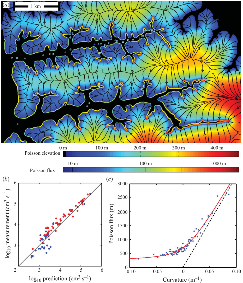
FIGURE 2. The water table and associated groundwater flux in the Florida network. (a) The magnitude of the Poisson flux (colour intensity on boundary) is the size of the area draining into a section of the network per unit length. It is found by solving (2.1) around the channels as approximated with an elevation contour. Flow lines are in black. The water discharge was measured at blue circles. The Poisson elevation and Poisson flux are proportional to the water table height and groundwater flux, respectively. (b) Comparison of the predicted discharge to measurements at 30 points in network taken in January 2009 (blue points) and 52 points in April 2009 (red points). The black line indicates equality. This comparison is direct and requires no adjustable parameters. (c) We observe a hyperbolic relationship between the curvature of the valley walls and the predicted flux (red curve). In regions of high curvature (i.e. valley heads) the flux is proportional to curvature (dashed line).
