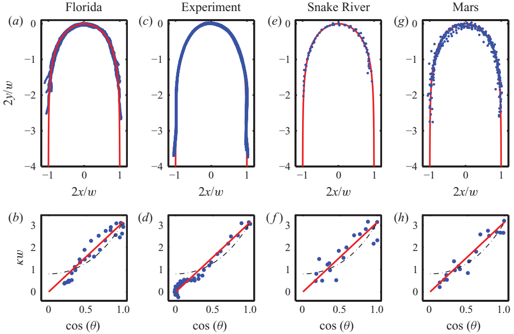
FIGURE 4. The shape of valley heads in the field, experiments, on Earth and on Mars are consistent with curvature-driven growth. (a) The shape of a channel produced by curvature-driven growth (red line) compared to the relative positions of points (blue dots) on the edge of valleys from the Florida network (17 elevation contours). (b) Comparison of the curvature at a point to the orientation (blue dots) of valleys from the Florida network. The red line is the linear relationship given in (6.1). The black dashed line corresponds to an ellipse with aspect ratio \pi . A semicircular head would predict the horizontal line \kappa w = 2 . (c–d) The analogous plots for the experiments (25 elevation contours extracted at 3 min intervals). (e–f) The analogous plots for three valleys near Box Canyon and Malad Gorge. (g–h) The analogous plots for 10 Martian ravines.
